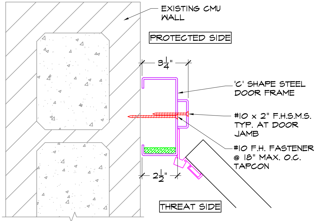
# STL. DOOR JAMB TO CMU WALL MADE W/10 GAUGE STEEL 3"=1'-0" SIM @ HEAD
